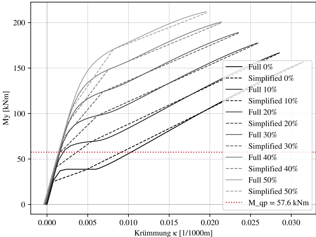
M-K-Diagrams at support of C1_2_1 — full vs. simplified, varying prestress
