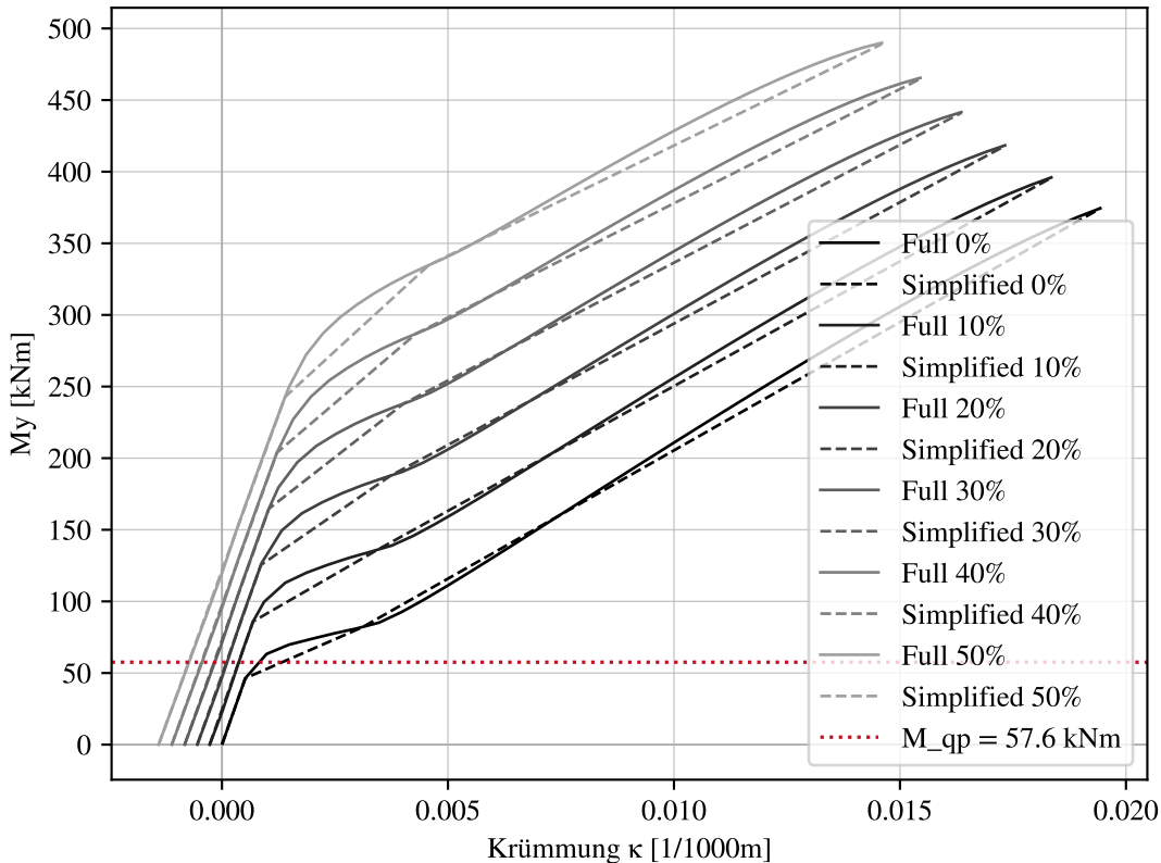
M-K-Diagrams at midspan of C1_3 — full vs. simplified, varying prestress
