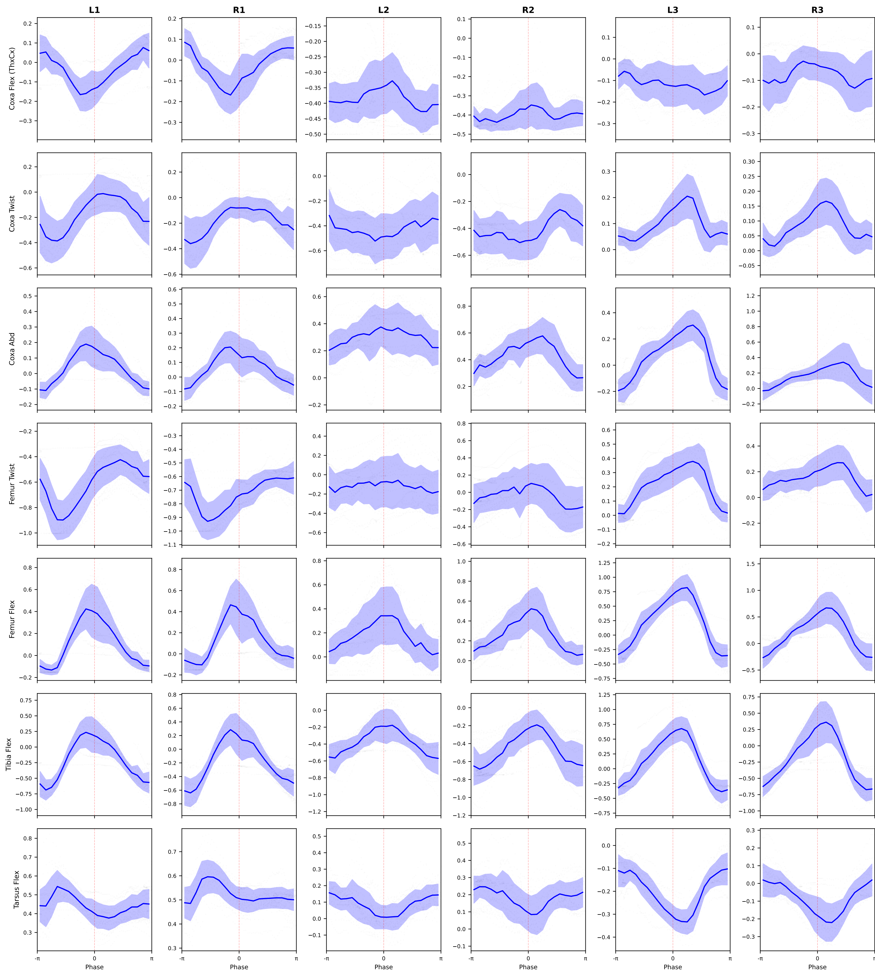
All Joint Angles vs Step Phase (7 joints × 6 legs)
