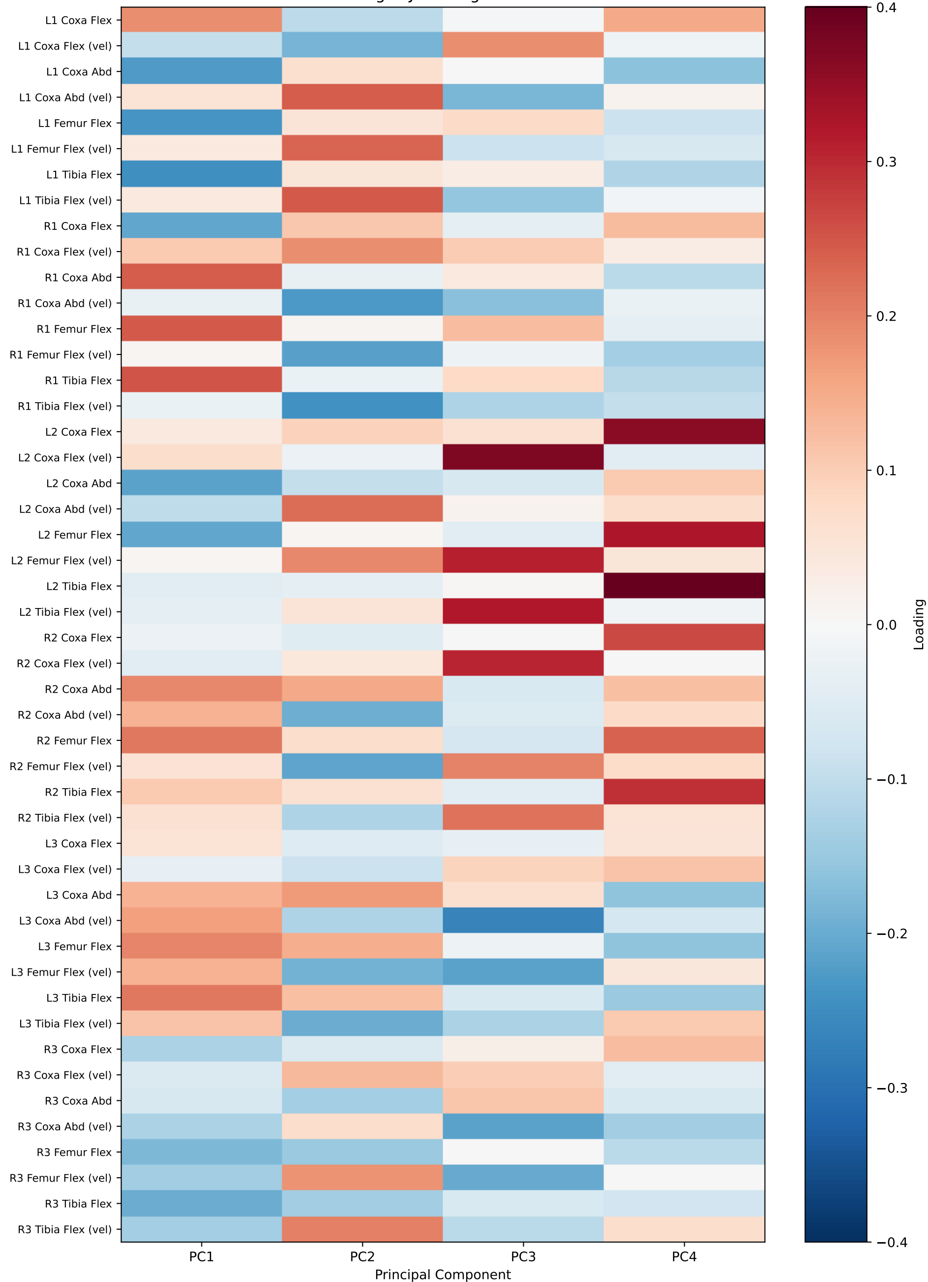
PCA Loadings - Joint Angles &amp; Velocities
