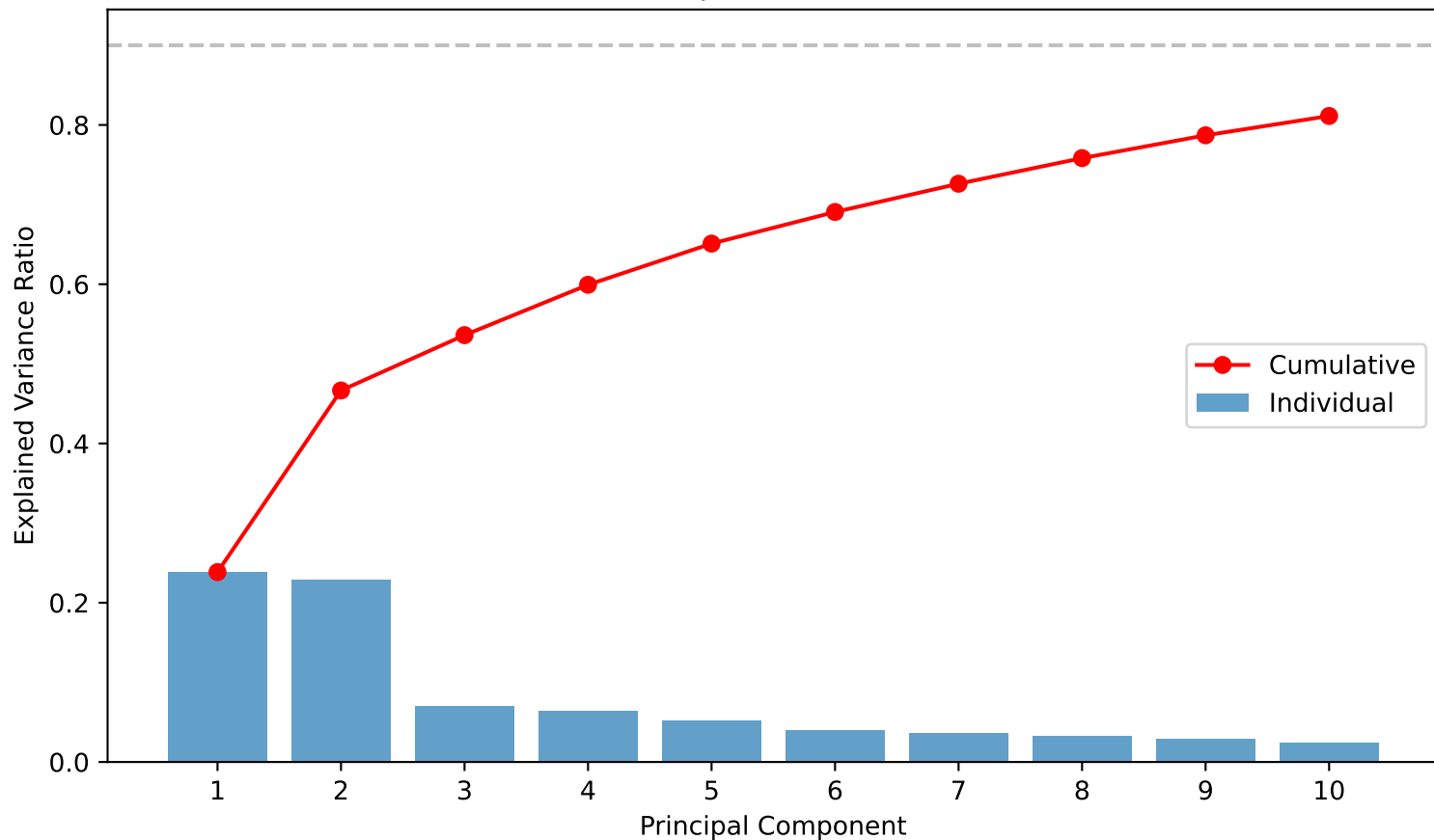
PCA Explained Variance
