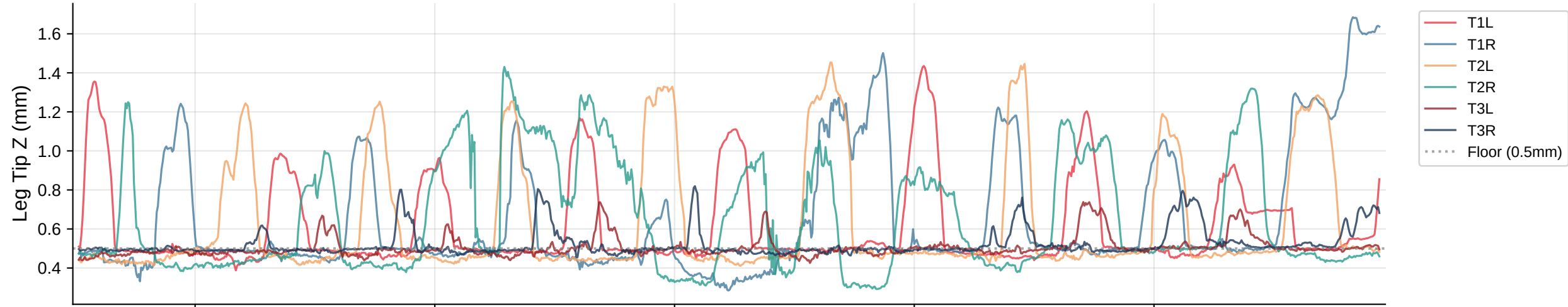
Leg Tip Z Trajectories | Bout 3
