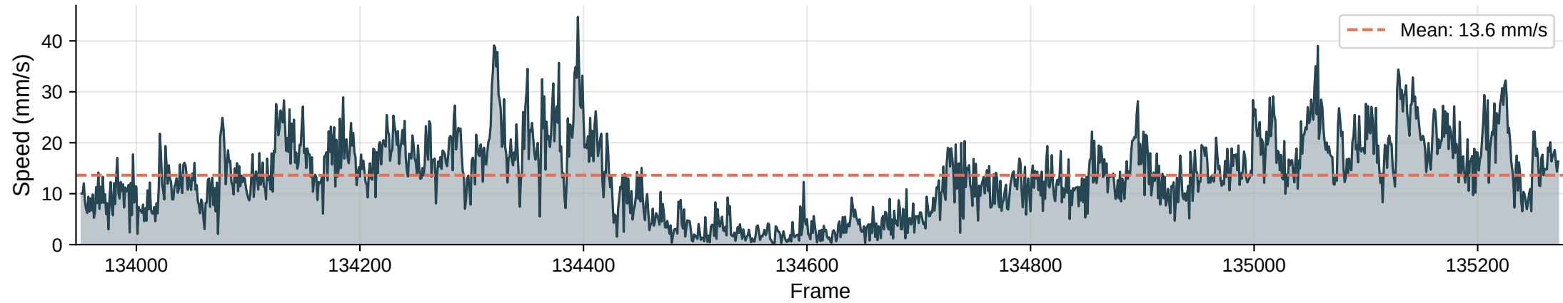
Instantaneous Speed | Max: 44.7 mm/s
