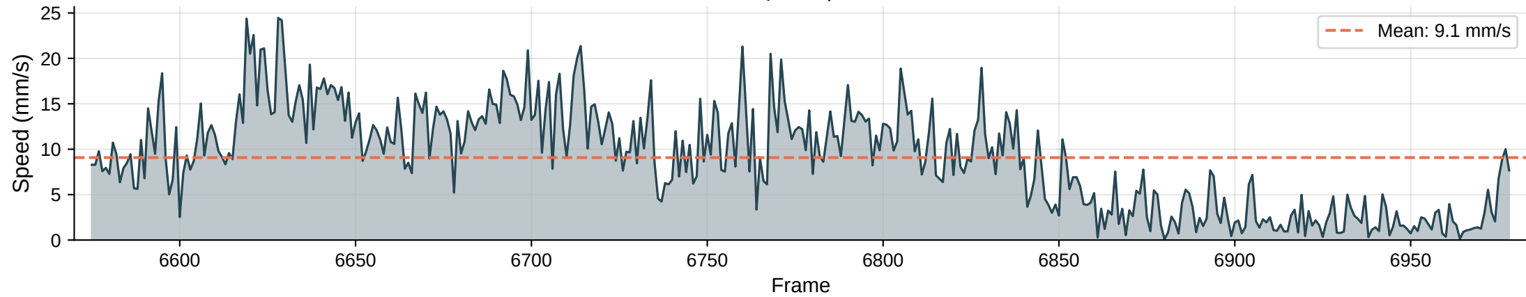
Instantaneous Speed | Max: 24.5 mm/s
