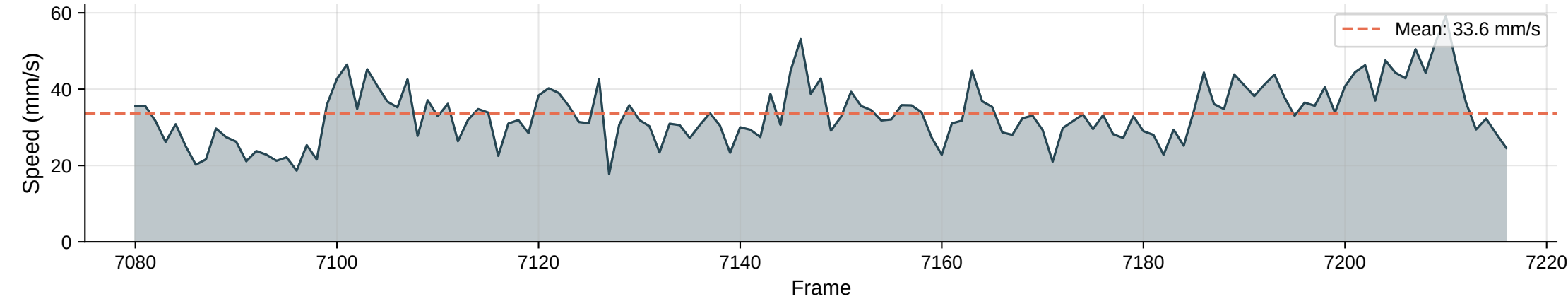
Instantaneous Speed | Max: 59.1 mm/s
