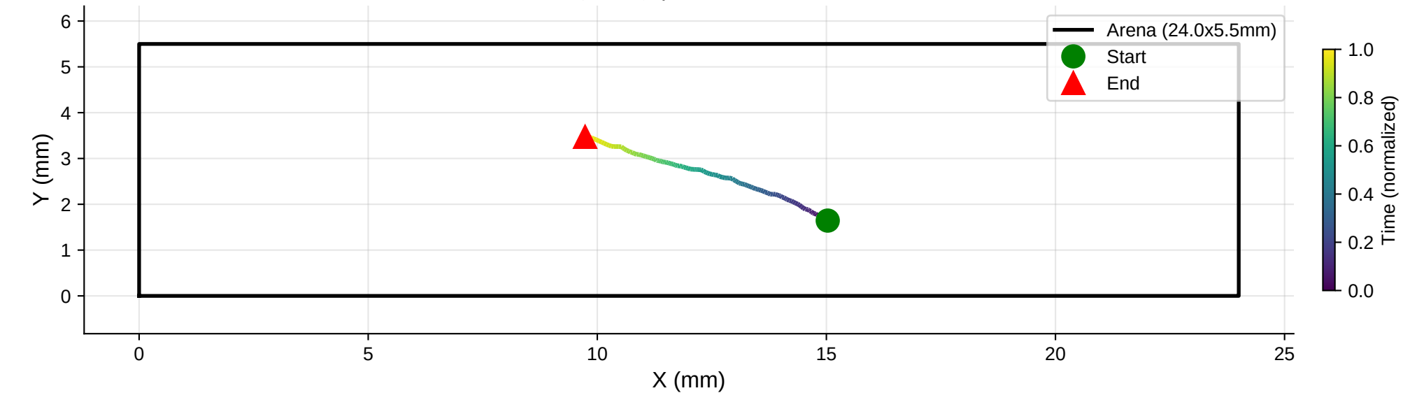
XY Trajectory | Distance: 5.70 mm
