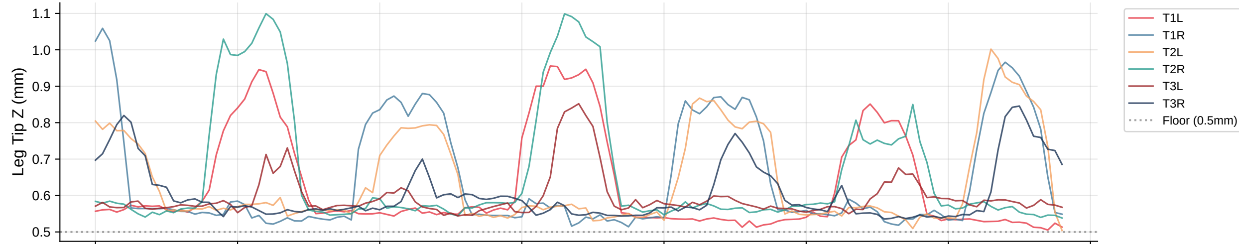
Leg Tip Z Trajectories | Bout 2
