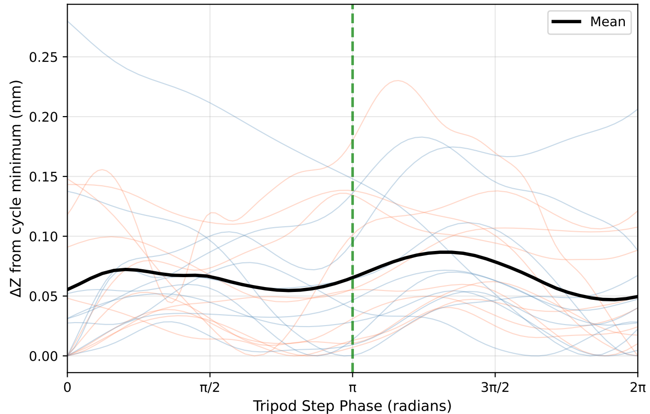
Individual Tripod Cycles (coral=left tripod, blue=right tripod)
