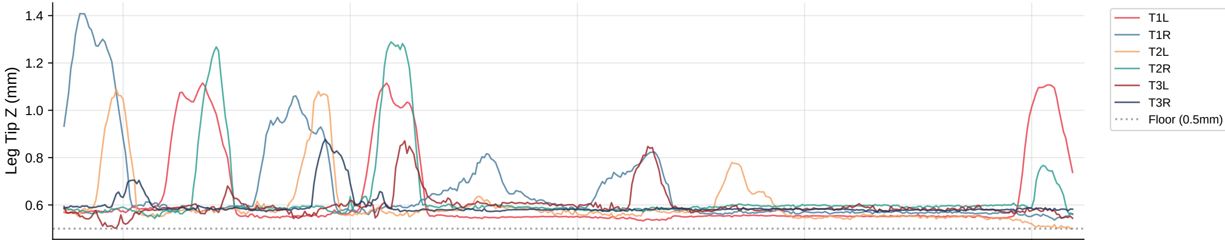
Leg Tip Z Trajectories | Bout 10
