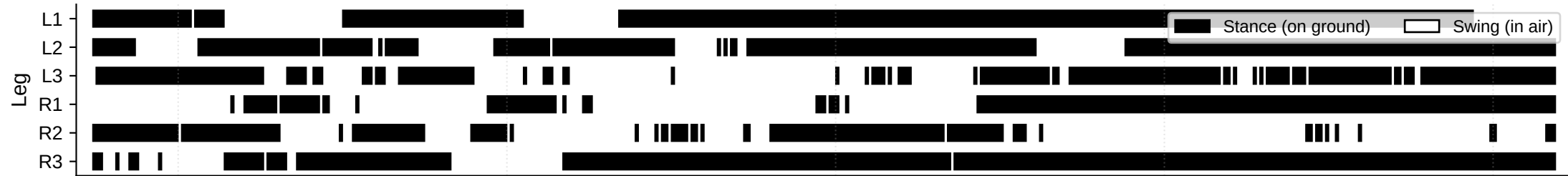
Gait Phase Diagram (black = stance, Z > 0.59mm)
