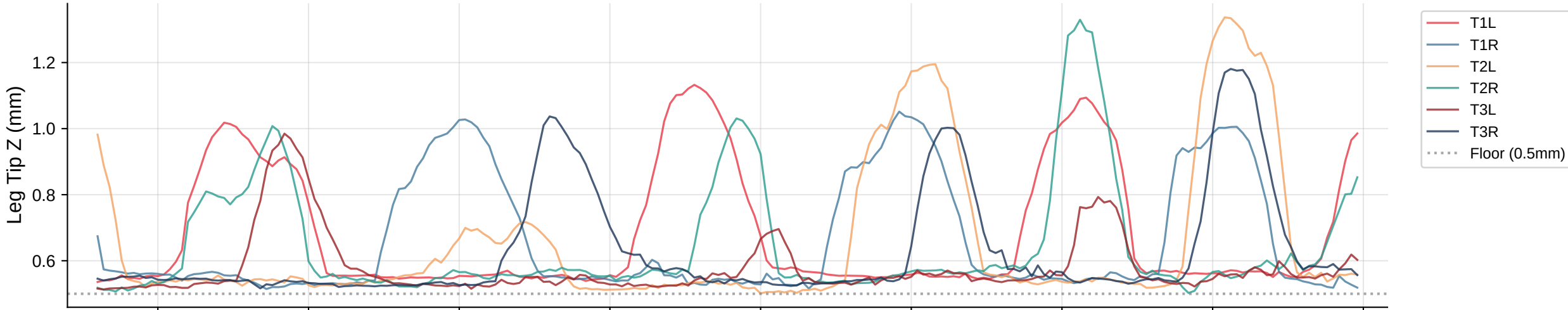
Leg Tip Z Trajectories | Bout 15
