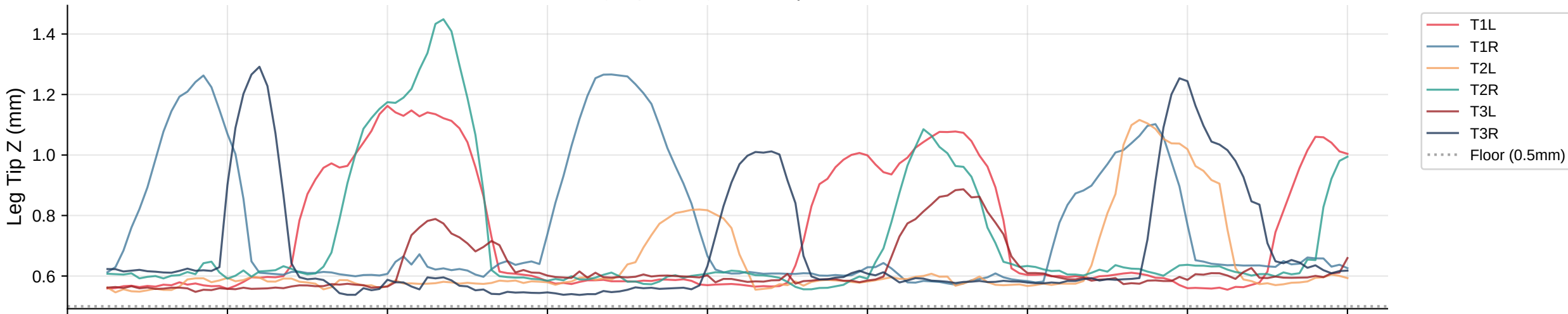
Leg Tip Z Trajectories | Bout 22
