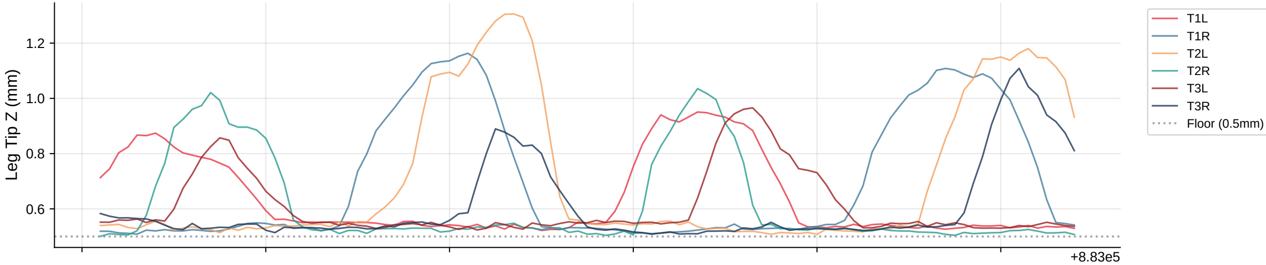
Leg Tip Z Trajectories | Bout 31
