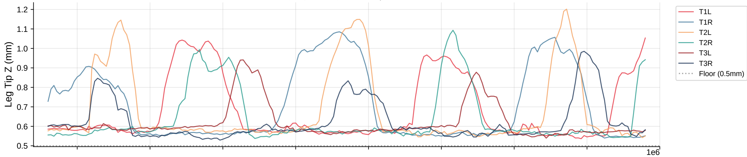
Leg Tip Z Trajectories | Bout 35
