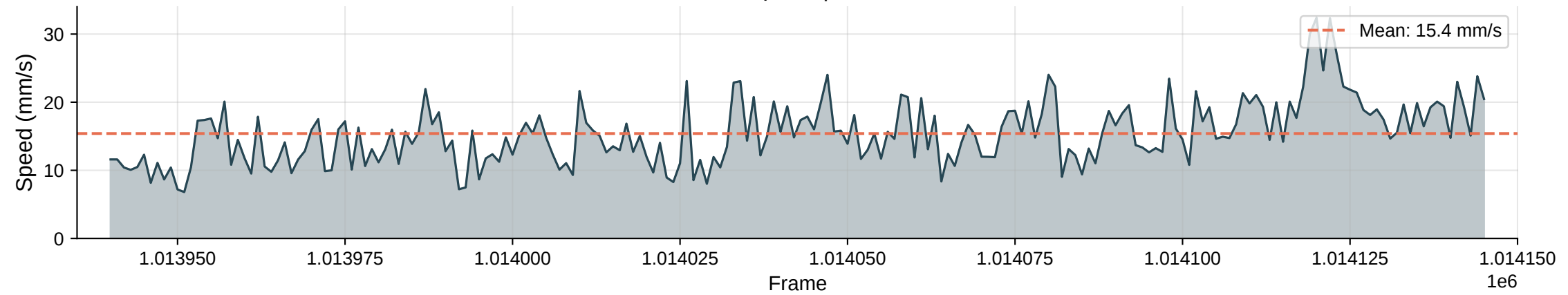
Instantaneous Speed | Max: 32.4 mm/s
