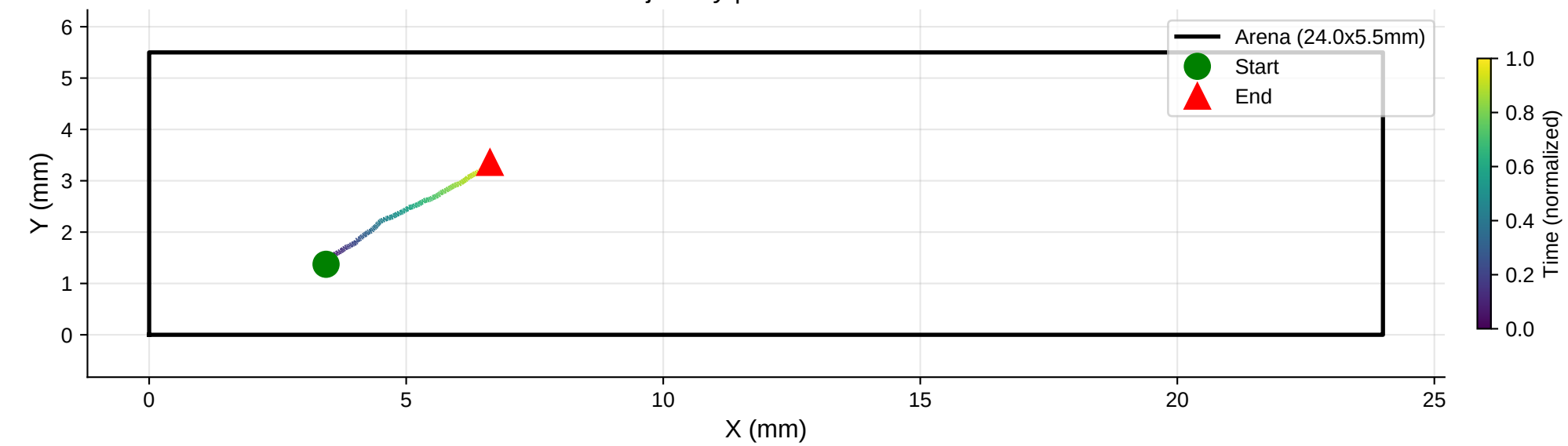
XY Trajectory | Distance: 3.95 mm
