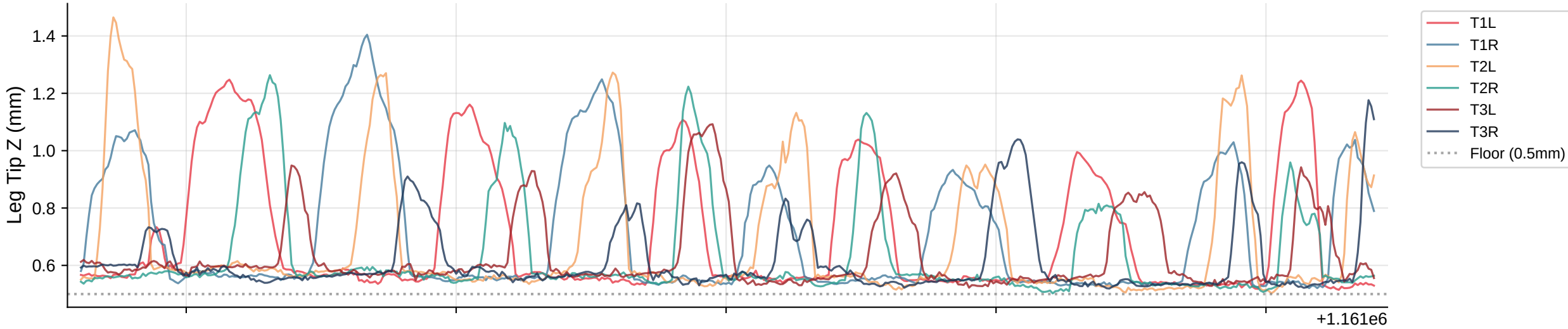
Leg Tip Z Trajectories | Bout 38
