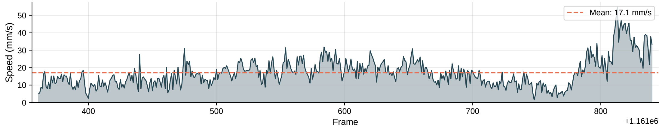
Instantaneous Speed | Max: 54.7 mm/s
