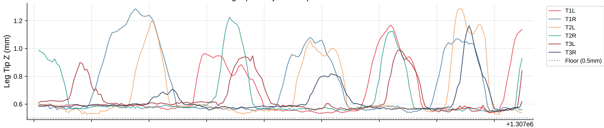
Leg Tip Z Trajectories | Bout 42
