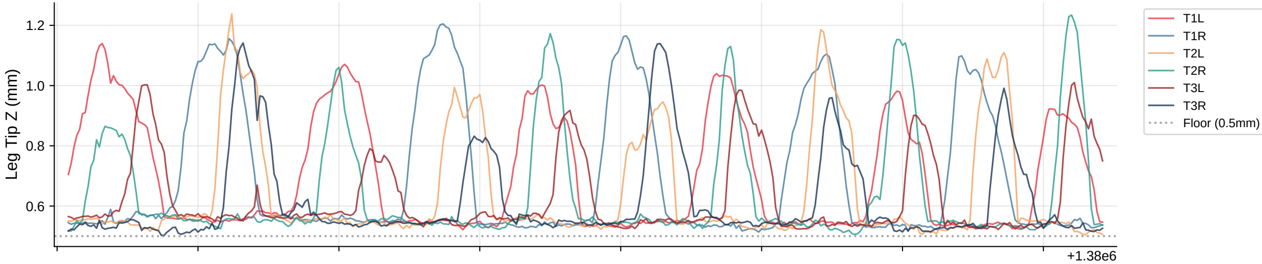
Leg Tip Z Trajectories | Bout 44
