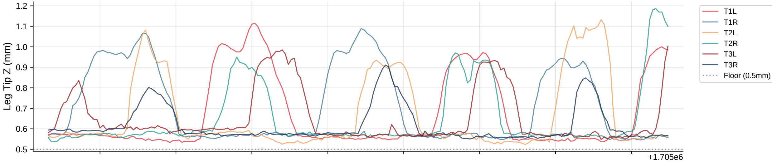
Leg Tip Z Trajectories | Bout 51
