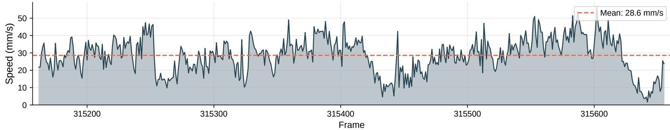
Instantaneous Speed | Max: 56.3 mm/s
