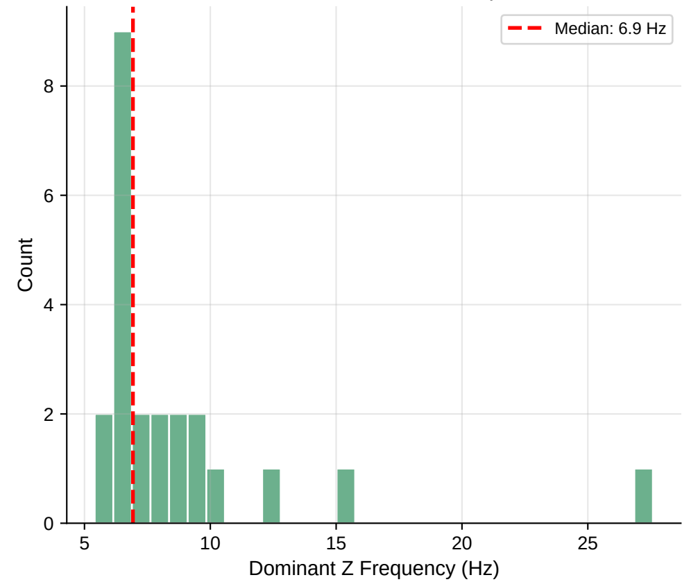
Distribution of Z Oscillation Frequencies
