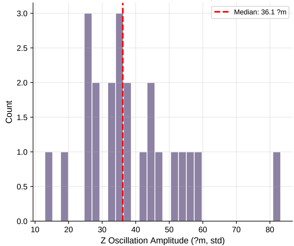
Distribution of Z Oscillation Amplitudes
