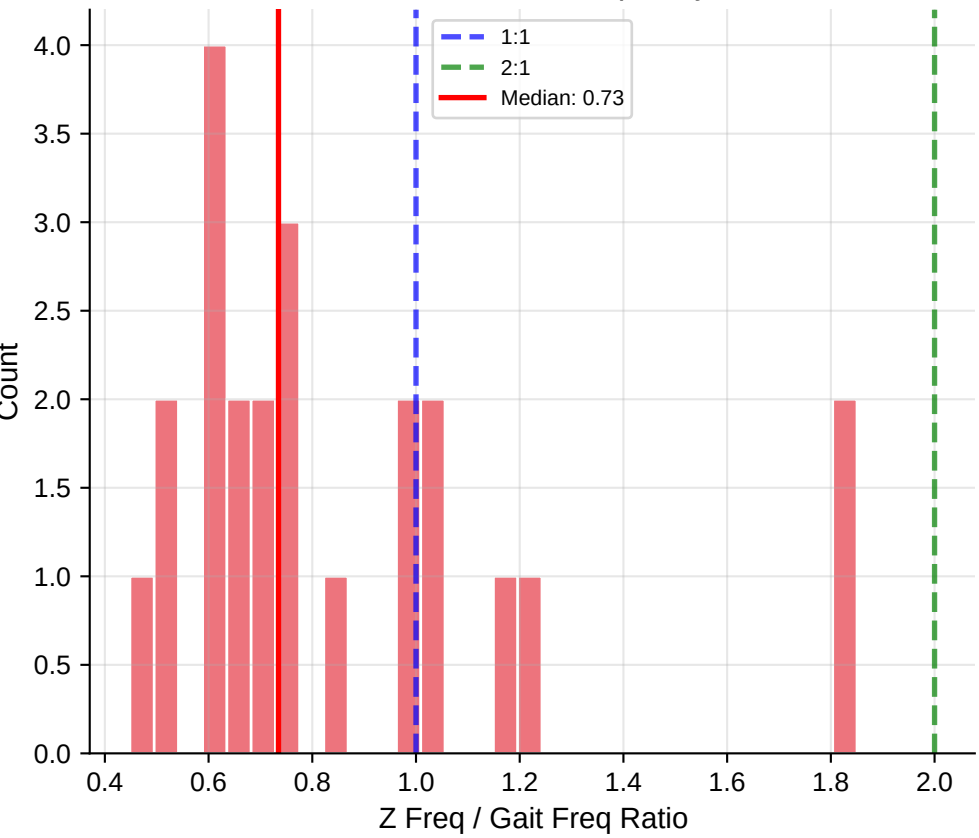
Z Oscillation to Gait Frequency Ratio
