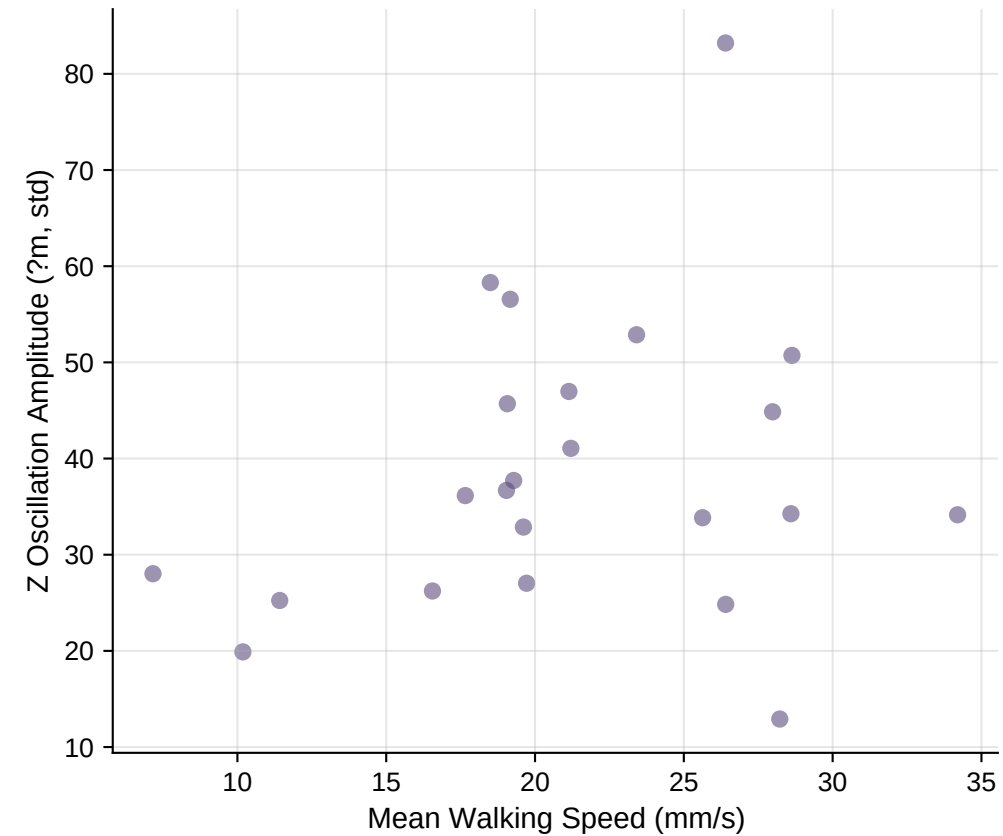
Speed vs Z Oscillation Pearson r = 0.235 , p = 2.81e-01
