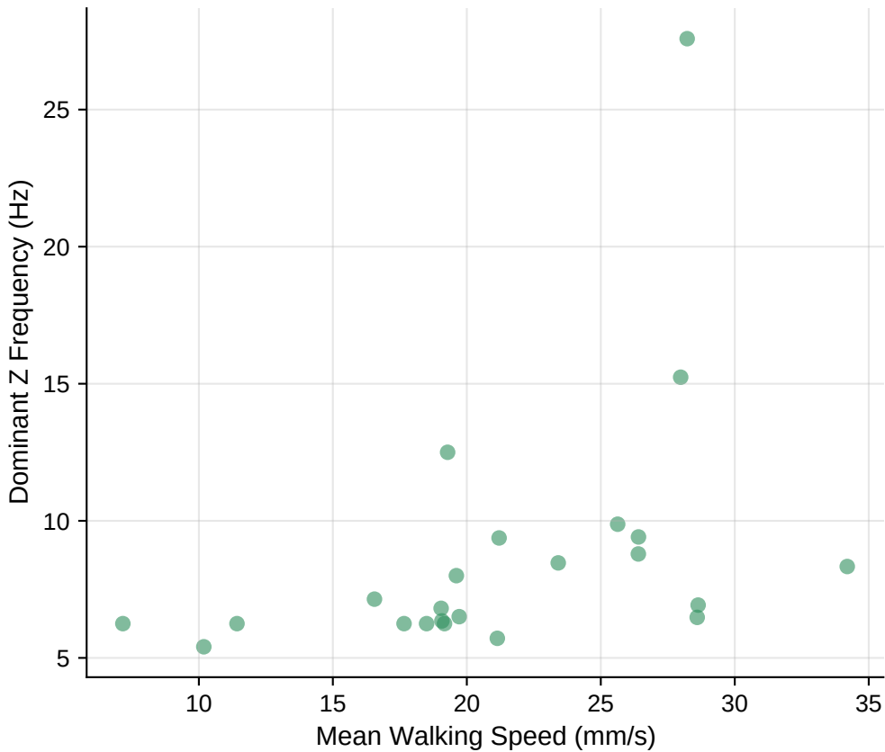
Speed vs Z Oscillation Frequency Pearson r = 0.414 , p = 4.94e-02
