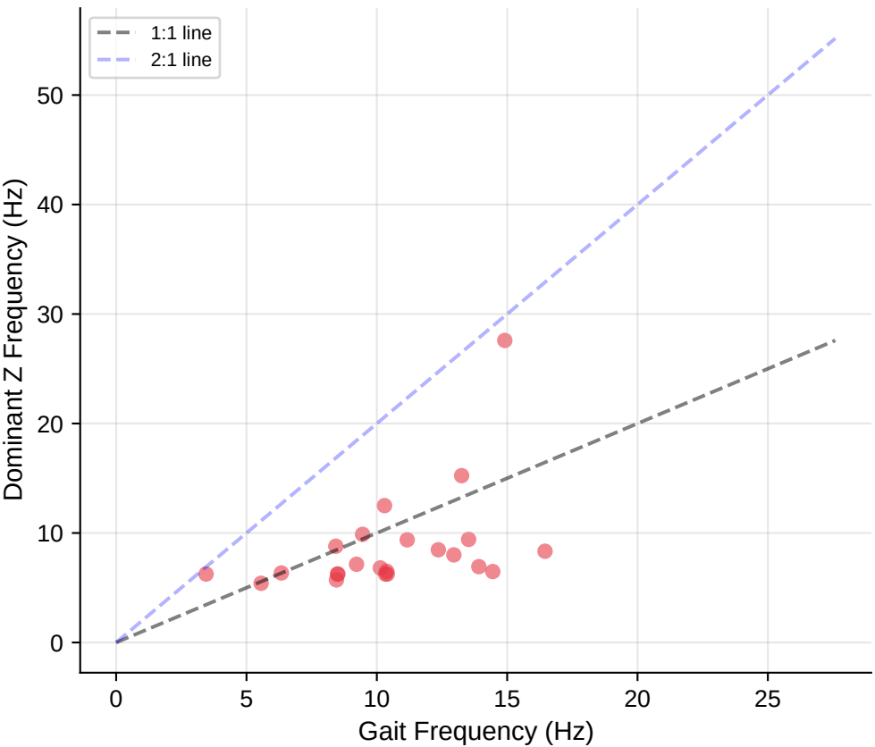
Gait vs Z Frequency Pearson r = 0.443 , p = 3.44e-02
