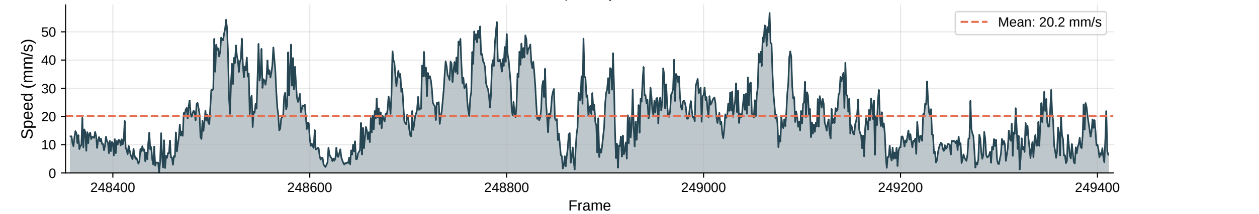
Instantaneous Speed | Max: 56.7 mm/s
