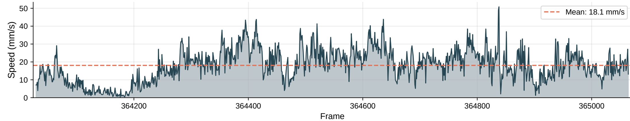
Instantaneous Speed | Max: 50.8 mm/s
