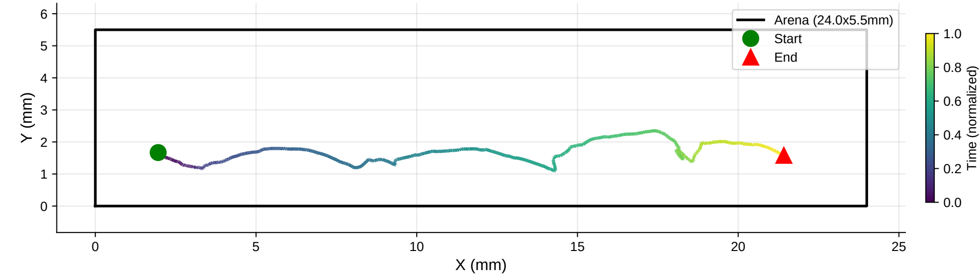
XY Trajectory | Distance: 23.38 mm
