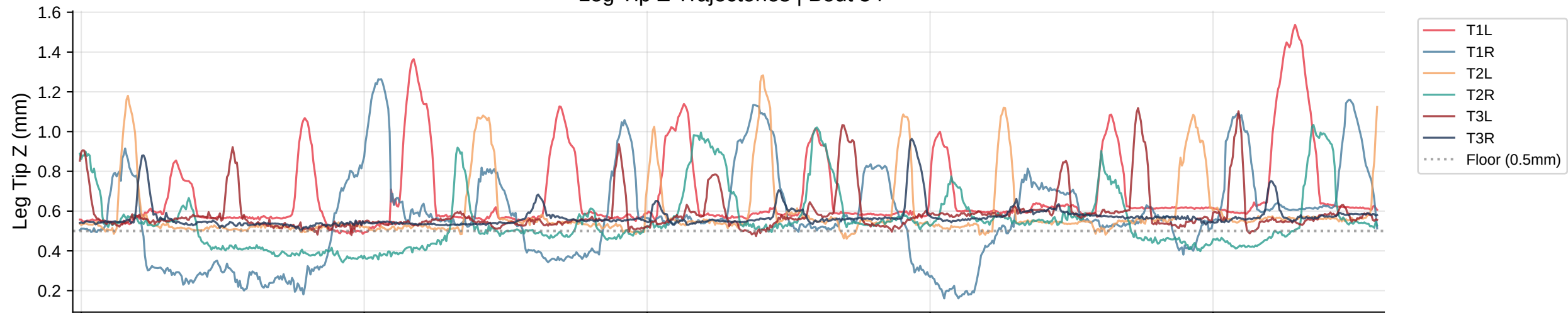
Leg Tip Z Trajectories | Bout 54
