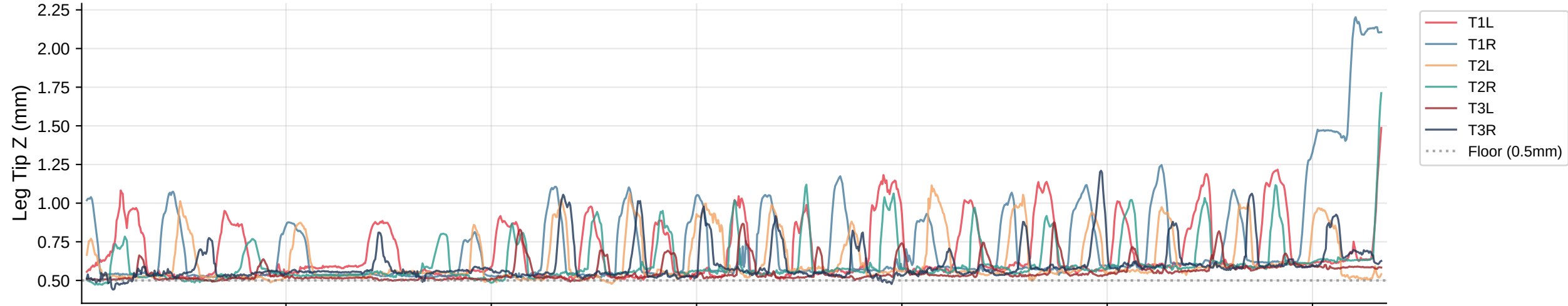
Leg Tip Z Trajectories | Bout 60
