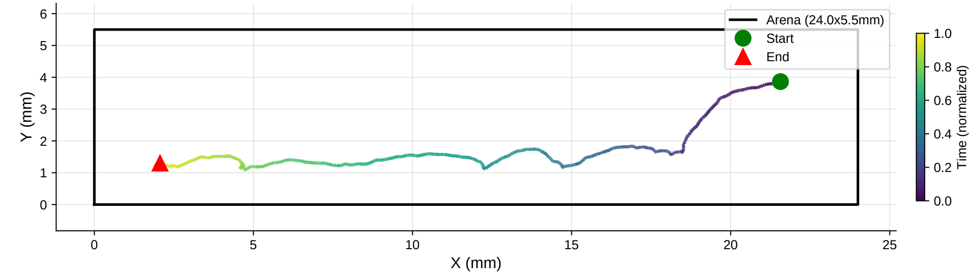
XY Trajectory | Distance: 23.96 mm
