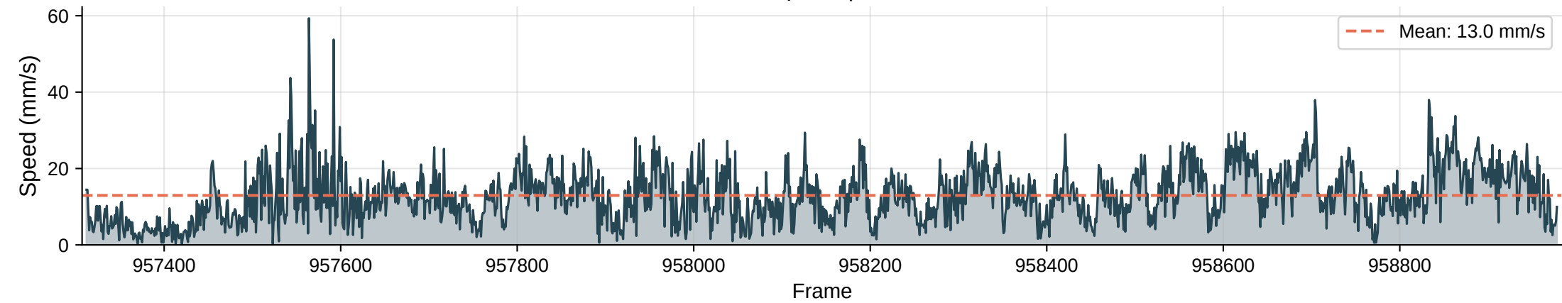
Instantaneous Speed | Max: 59.3 mm/s
