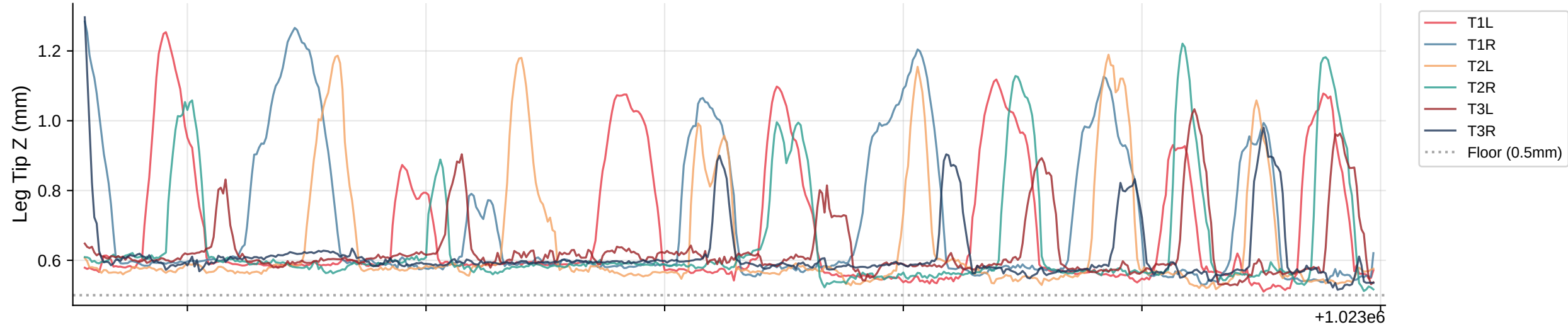
Leg Tip Z Trajectories | Bout 87
