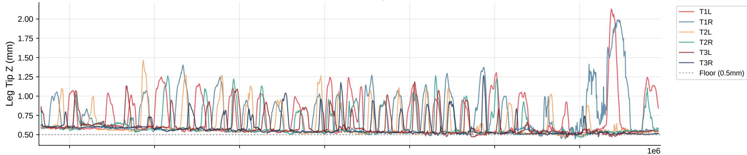
Leg Tip Z Trajectories | Bout 93
