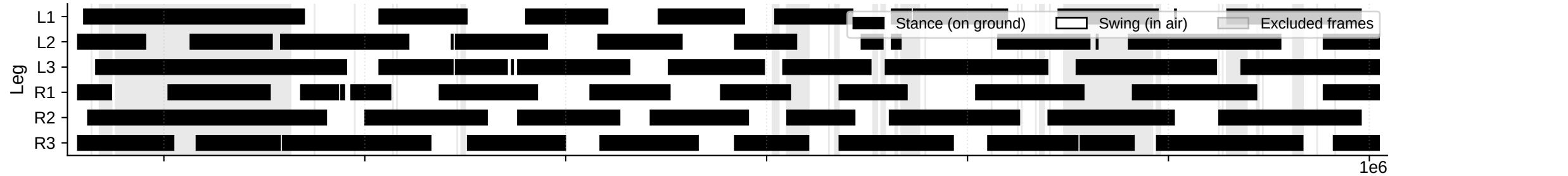
Gait Phase Diagram (black = stance, Z > 0.59mm)
