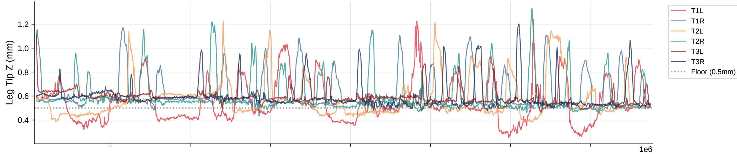
Leg Tip Z Trajectories | Bout 128
