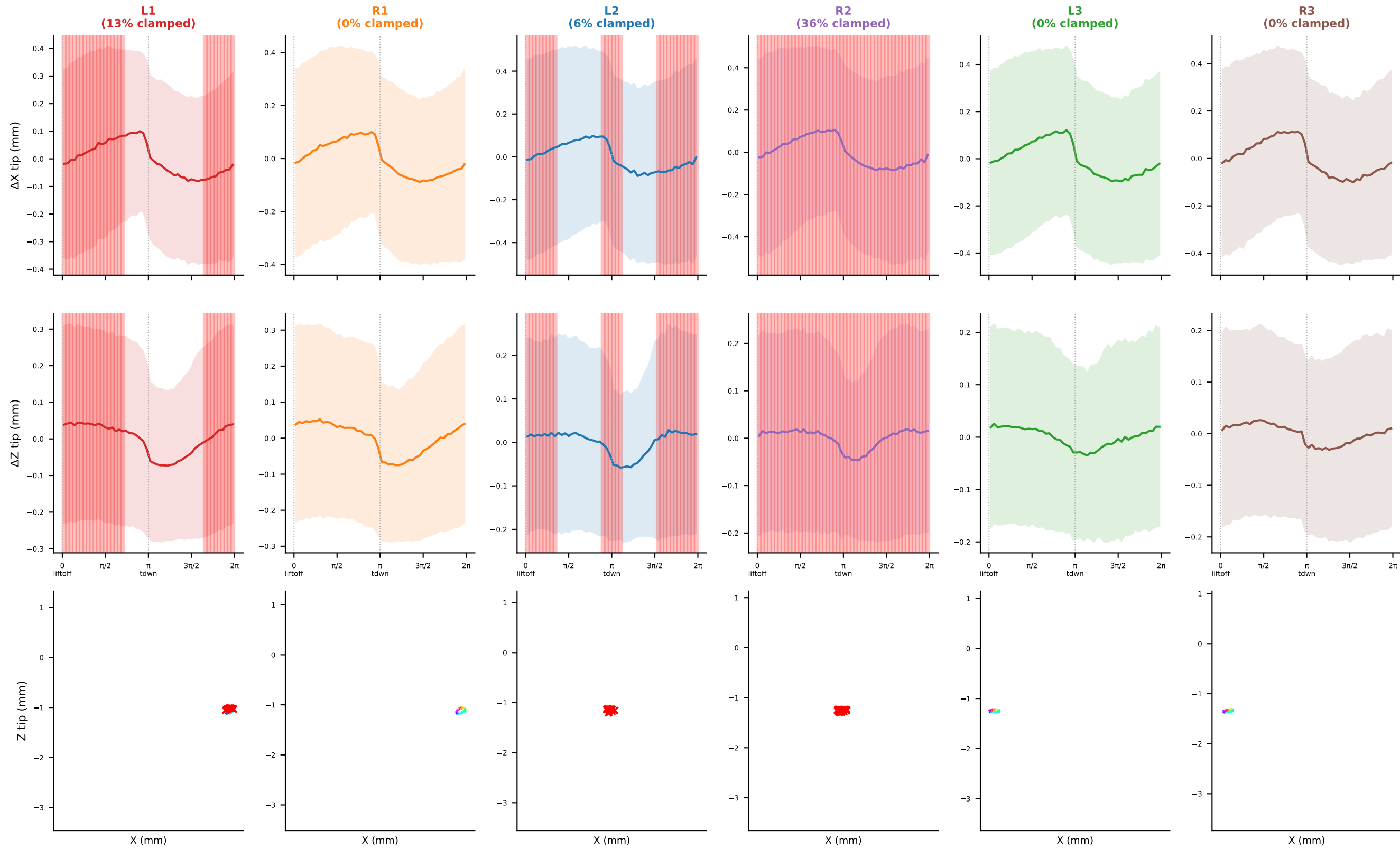
Leg tip egocentric position vs step phase | red shading = bins where >5% frames have coxa_twist clamped Row 3: XZ arc per leg (phase colormap 0→2π; red x = clamped bins)
