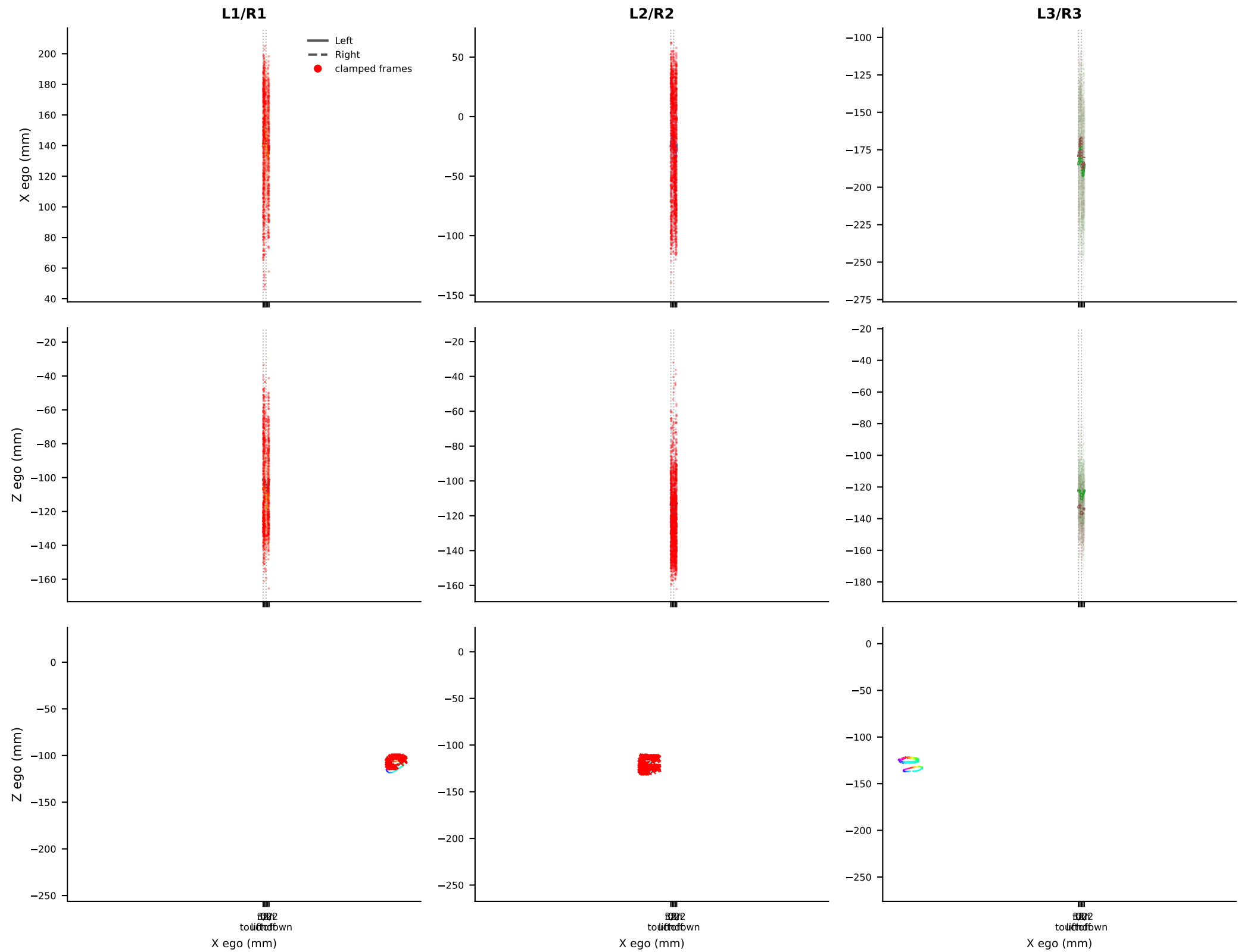
Leg tip egocentric position vs step phase | red = coxa_twist clamped at joint limit Row 3: XZ step arc (colored by phase 0→2π, red × = clamped bins)
