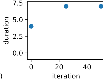
Median duration
