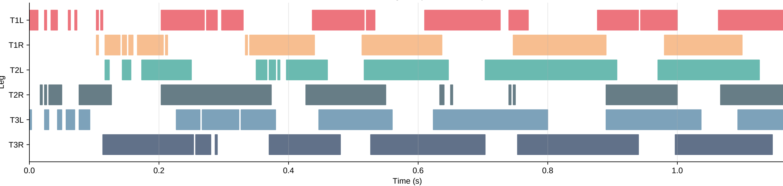
Gait Phase Diagram (filled = stance)
