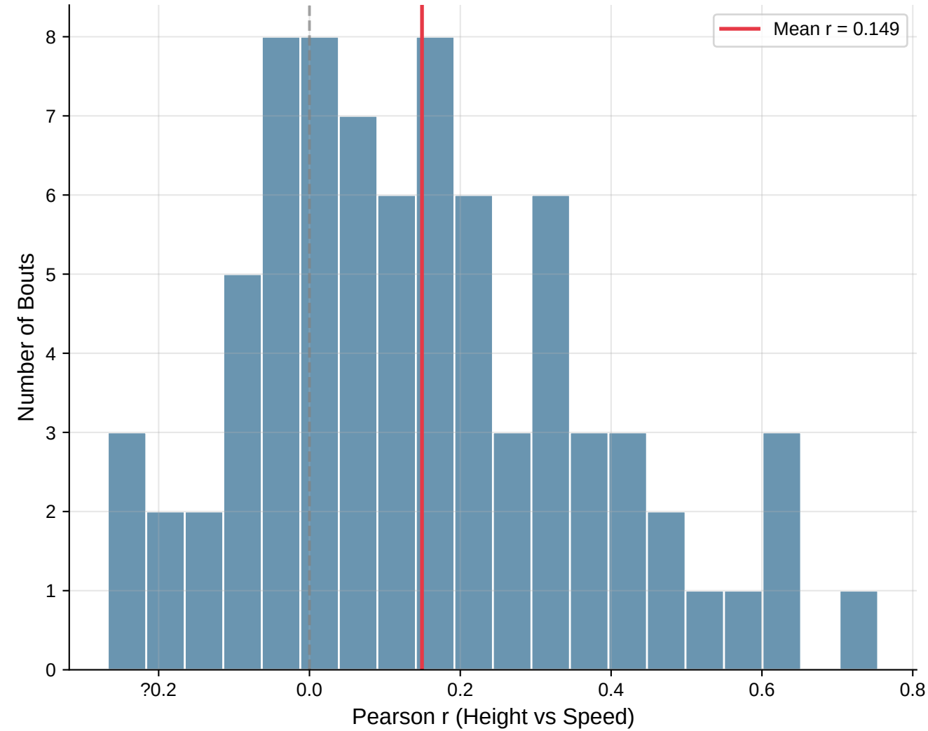
Distribution of Within-Bout Correlations (n=78)
