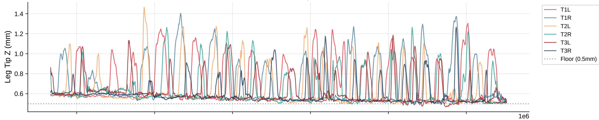
Leg Tip Z Trajectories | Bout 5
