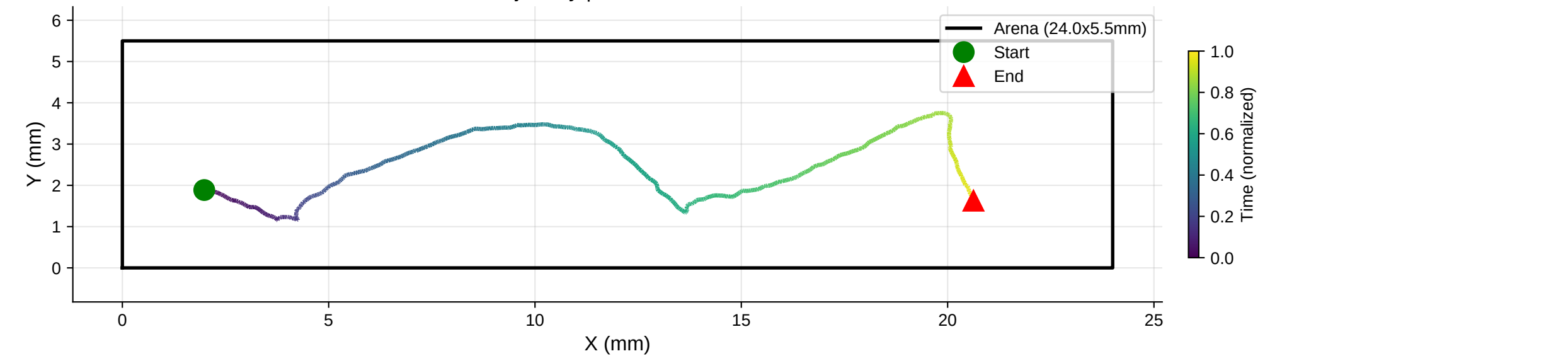
XY Trajectory | Distance: 23.85 mm
