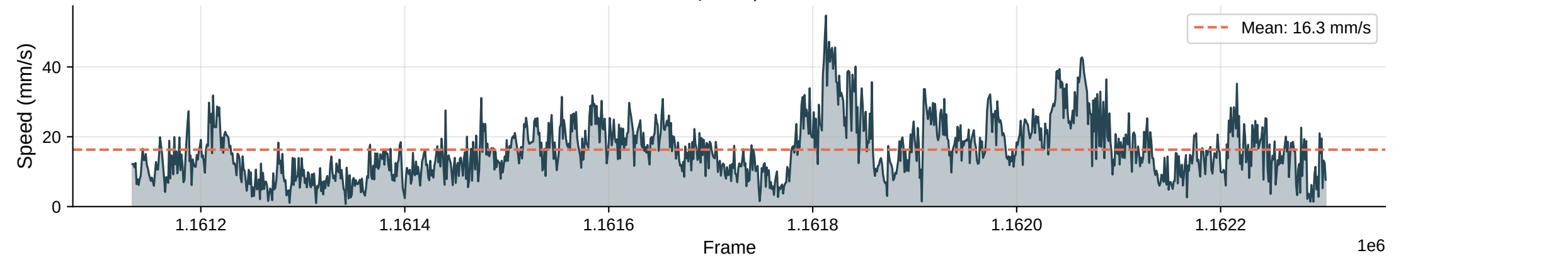
Instantaneous Speed | Max: 54.7 mm/s
