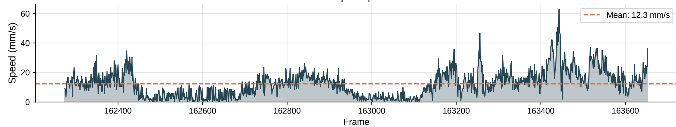
Instantaneous Speed | Max: 63.0 mm/s
