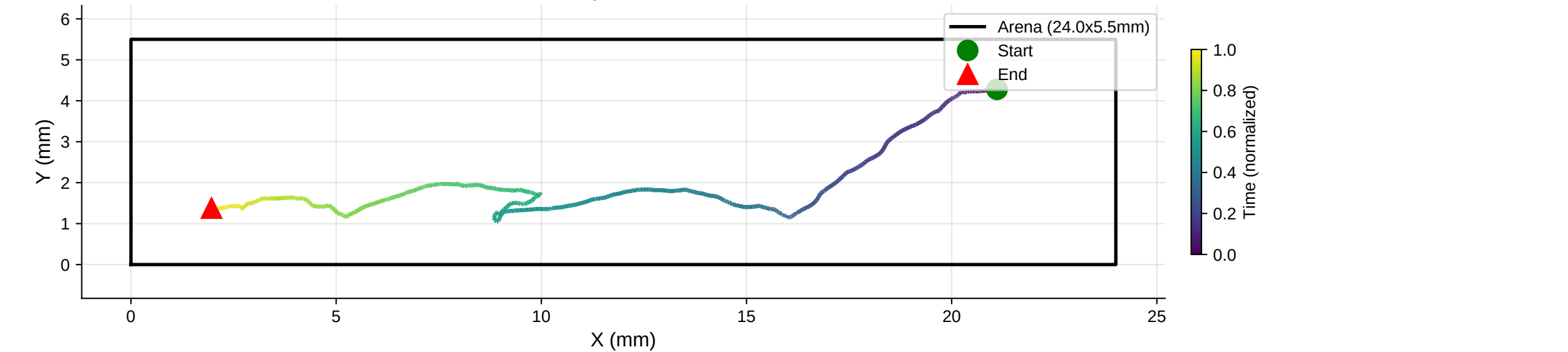
XY Trajectory | Distance: 24.30 mm
