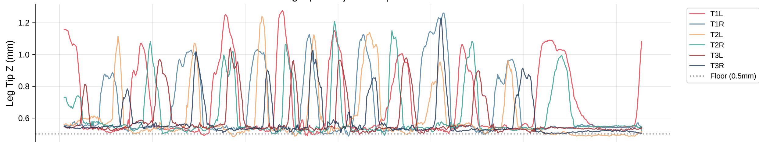
Leg Tip Z Trajectories | Bout 32
