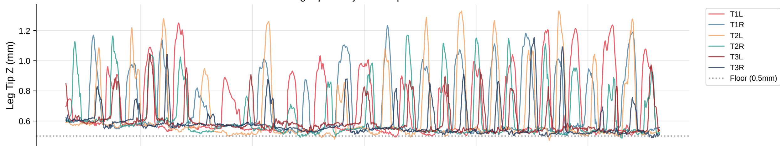
Leg Tip Z Trajectories | Bout 33
