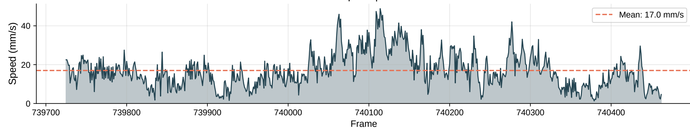
Instantaneous Speed | Max: 48.9 mm/s
