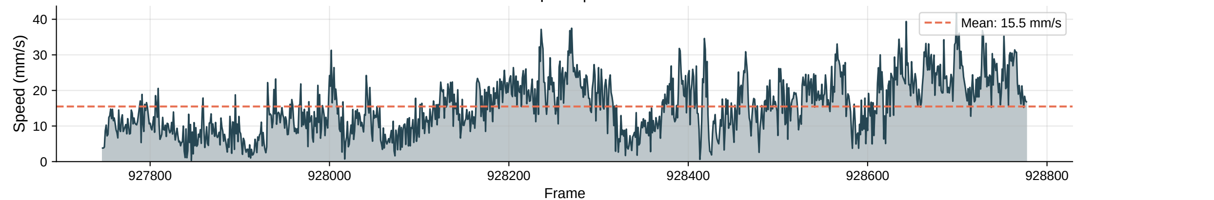
Instantaneous Speed | Max: 41.6 mm/s
