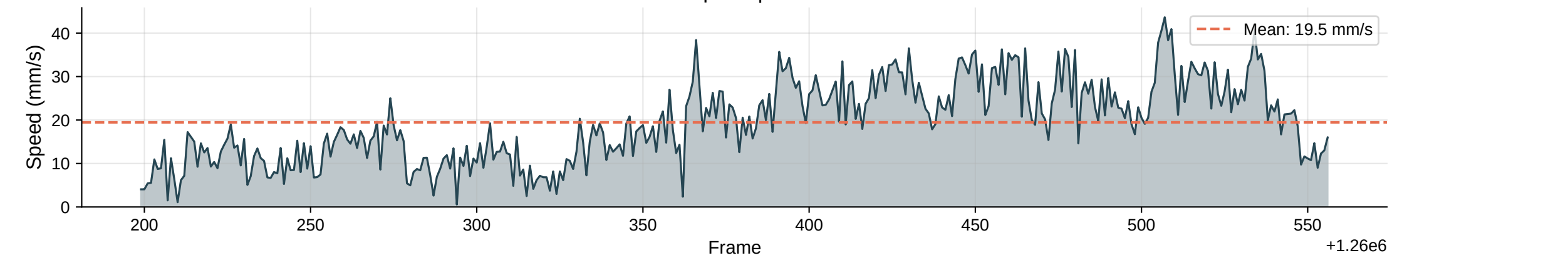
Instantaneous Speed | Max: 43.6 mm/s
