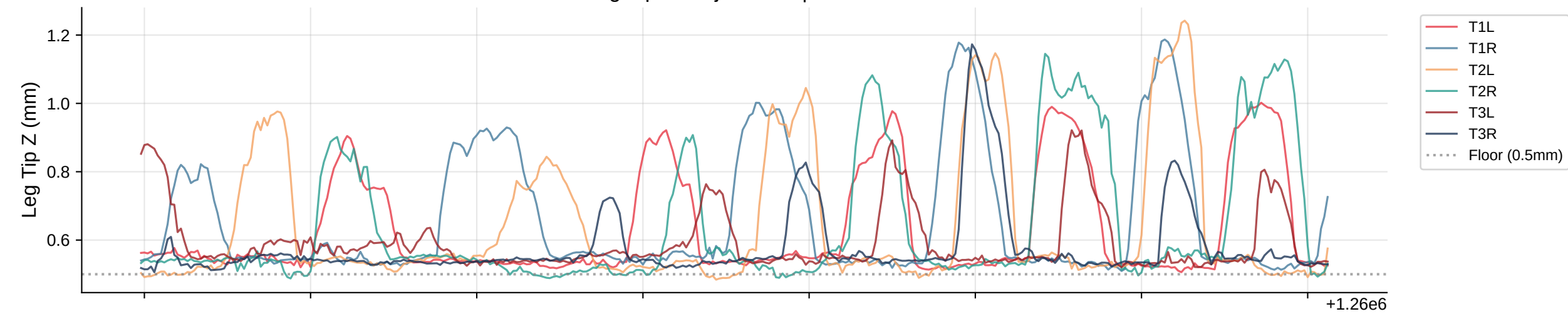
Leg Tip Z Trajectories | Bout 60
