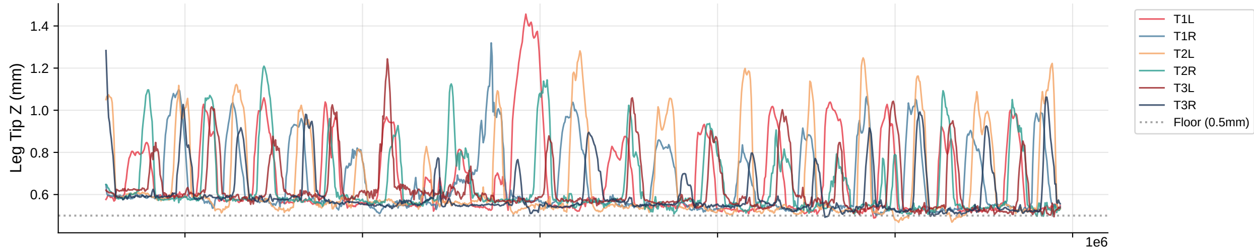
Leg Tip Z Trajectories | Bout 68
