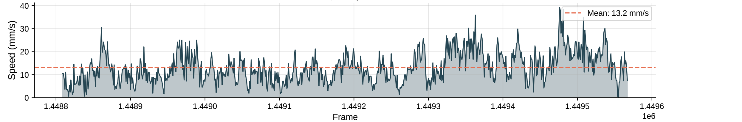
Instantaneous Speed | Max: 39.3 mm/s
