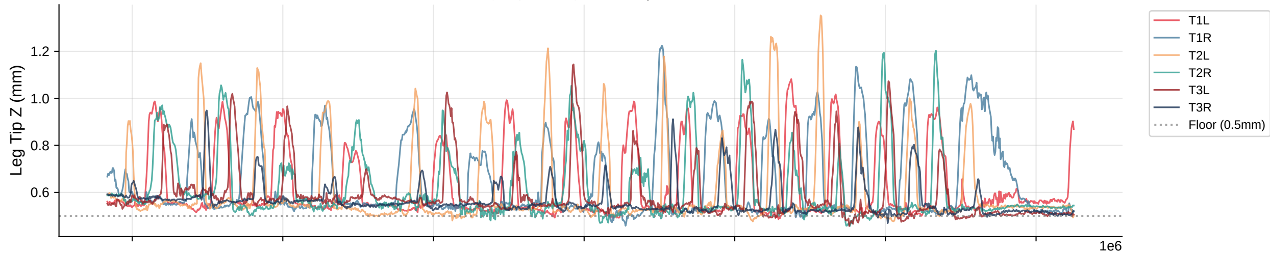
Leg Tip Z Trajectories | Bout 77
