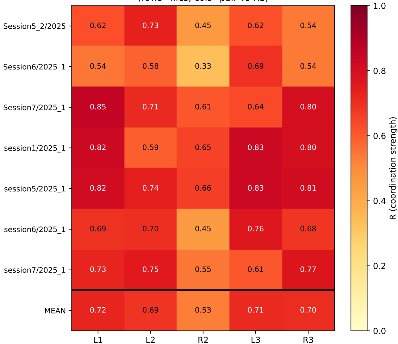
Onset-based coordination R (rows=flies, cols=pair vs R1)
