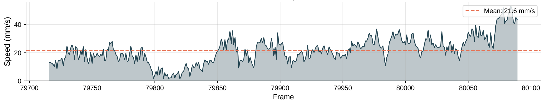
Instantaneous Speed | Max: 53.1 mm/s
