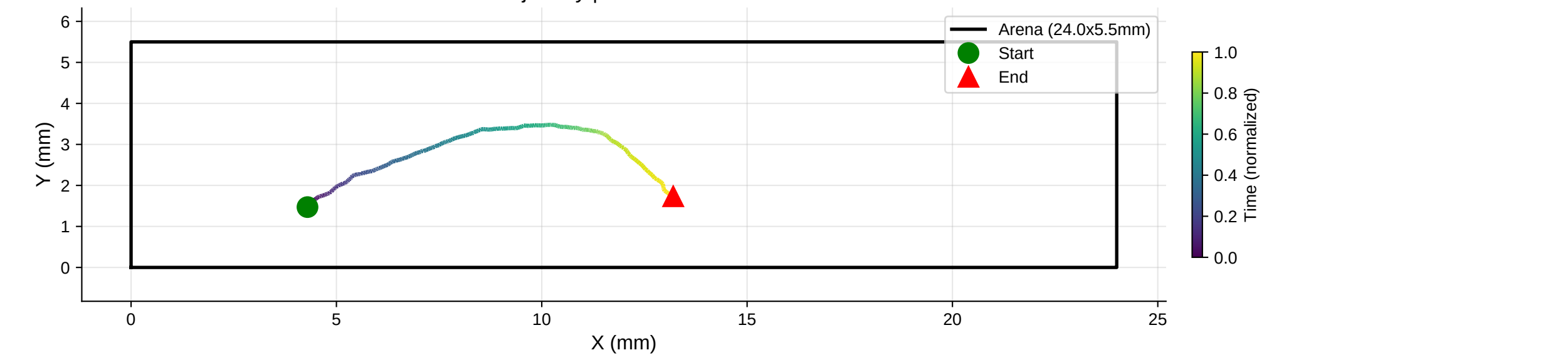
XY Trajectory | Distance: 10.26 mm
