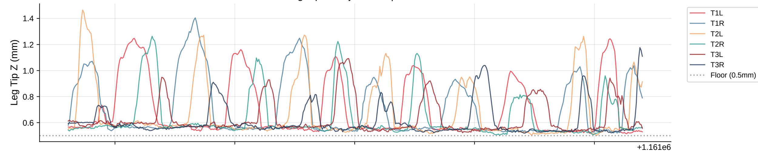
Leg Tip Z Trajectories | Bout 2
